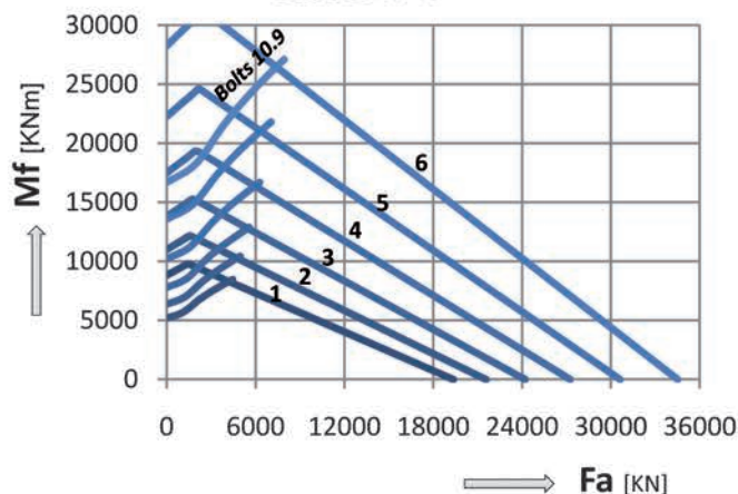
Curves 1~6
